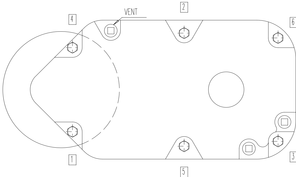
Figure 1 – Frame 1 or TR3 Bolt-tightening Sequence
