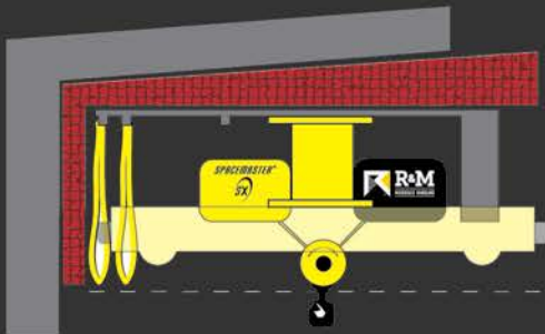
Figure 1. C-track Festoon
