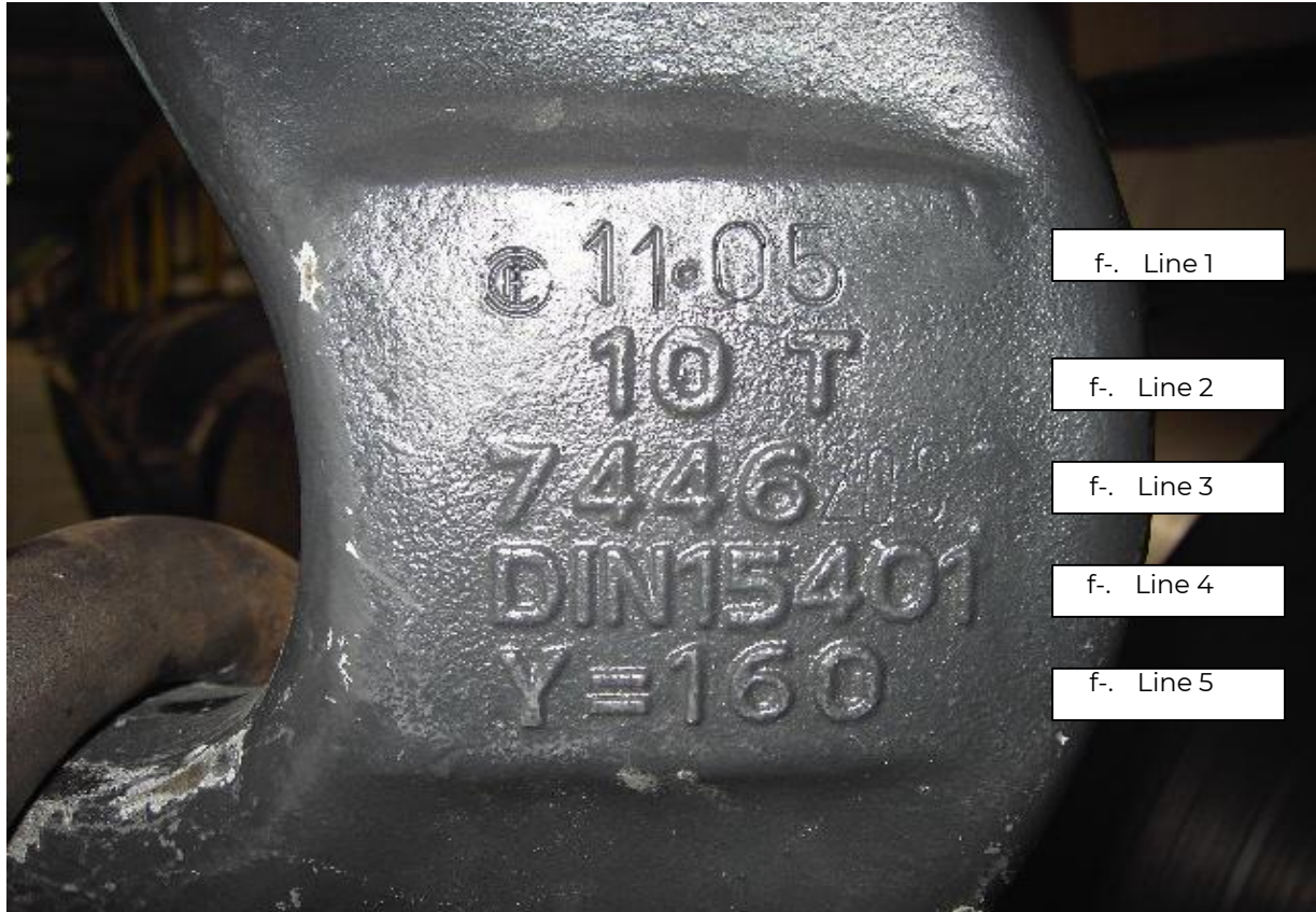
An example of markings on an RSN10 size load hook.
