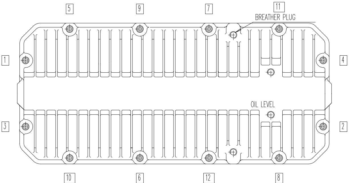
Figure 1 – Frame D Bolt-tightening Sequence
